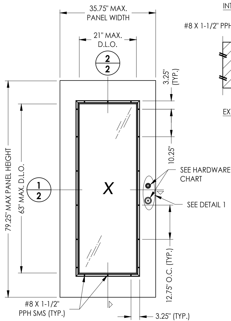
40 41 DOOR AND SIDELITE PANEL #40 - Steel Edge Steel Door #41 - Steel Edge Sidelite
