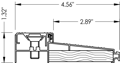
30 INSWING THRESHOLD
