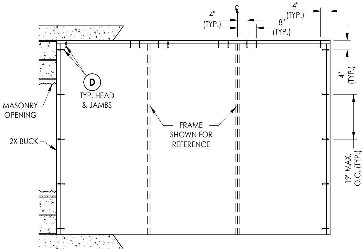
BUCK ANCHORING
