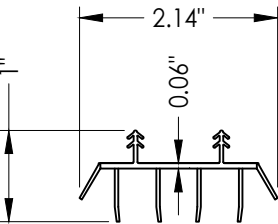
6 SWEEP
