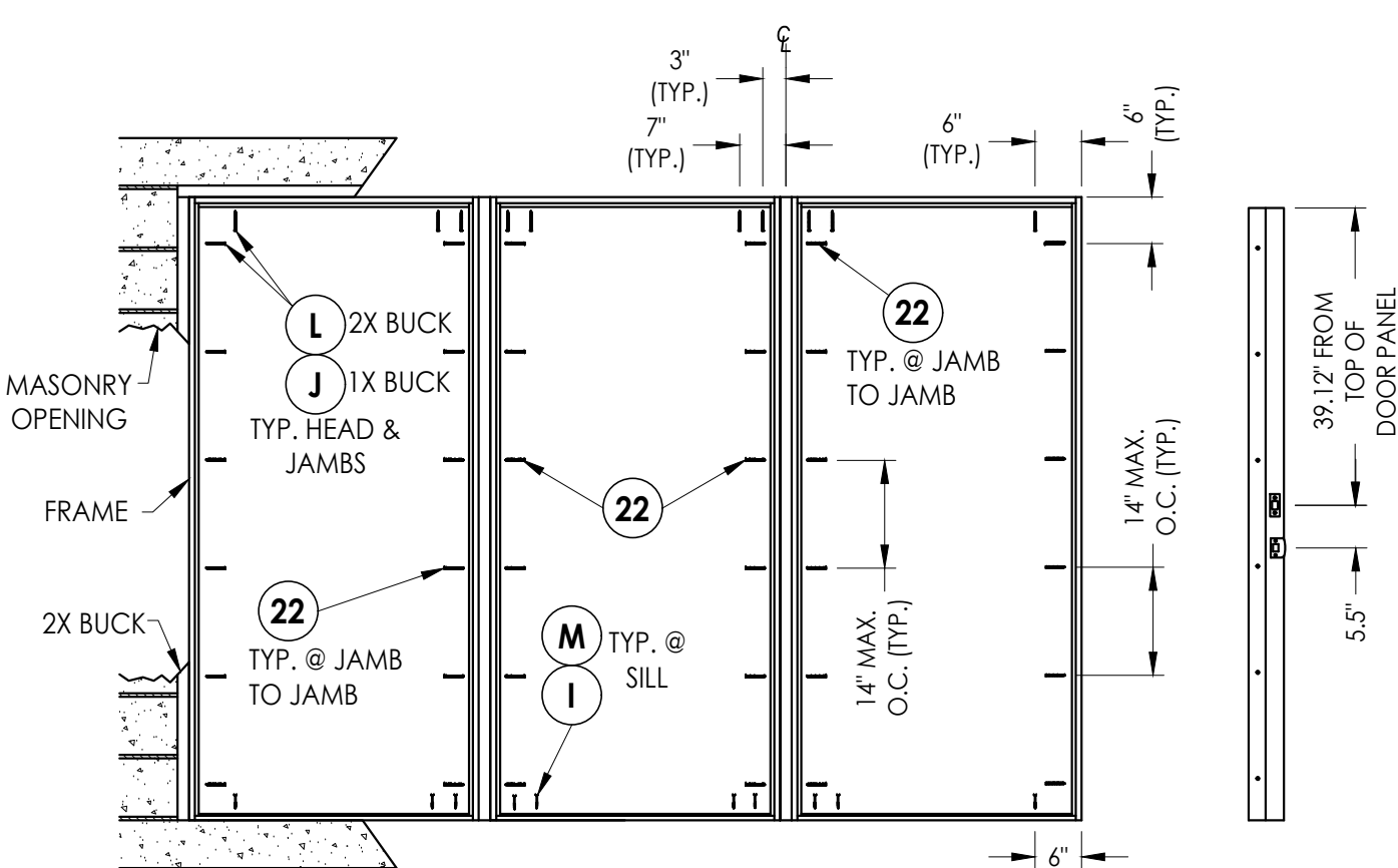
FRAME ANCHORING
