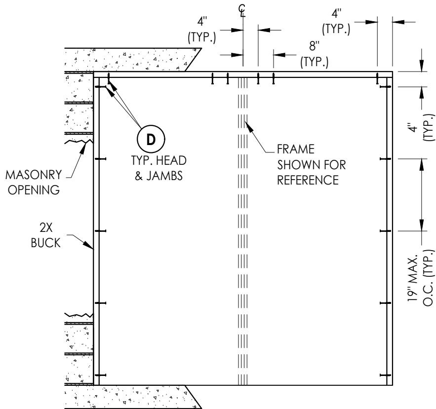
BUCK ANCHORING
